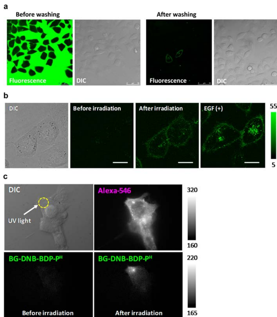
Figure 3. Optical highlighting of EGFR-SNAP fusion protein. (a) Confocal fluorescence image of BG-Bn-BDP-P H (10, 2 μM)-loaded HeLa cells transiently expressing EGFR-SNAP protein before washing (left panel) and after washing (right panel). (b) Confocal fluorescence image of BG-DNB-BDP-P H (9, 2 μM)-loaded HeLa cells transiently expressing EGFR-SNAP protein before and after UV irradiation. UV irradiation was carried out at the whole field for 5 min by a handy-held UV lamp (365 nm, 1.5 mW/cm 2 ). After EGF addition to the irradiated cell culture (final concentration: 100 ng/mL) and incubation at 37 °C for 3 h, a fluorescence image was captured. Scale bar: 15 μm. (c) Epifluorescence images of BG-DNB-BDP-P H (2 μM)-loaded COS-7 cells transiently expressing EGFR-SNAP protein before and after UV irradiation. Localized UV irradiation was carried out for 30 s through an objective lens with a pinhole. EGFR-SNAP expressing cells were marked with a cell-impermeable fluorescent marker, BG-Alexa-546 (2 μM), after labeling with BG-DNB-BDP-P H (2 μM).
